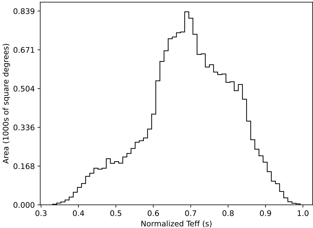
weather_cloudso0v3.5_10yrs WFD all bands: Normalized Teff
