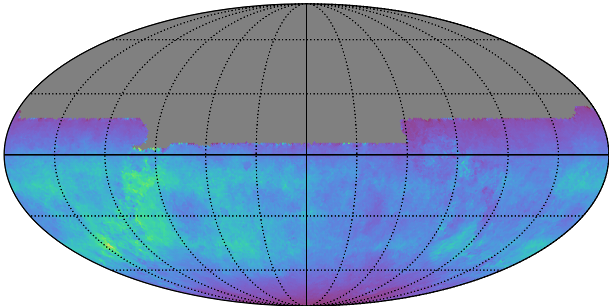
weather_cloudso0v3.5_10yrs All sky u band: Normalized Teff
