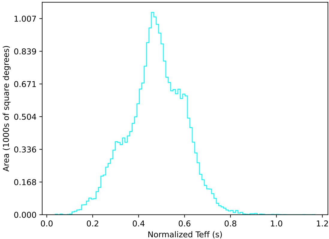
weather_cloudso0v3.5_10yrs All sky u band: Normalized Teff
