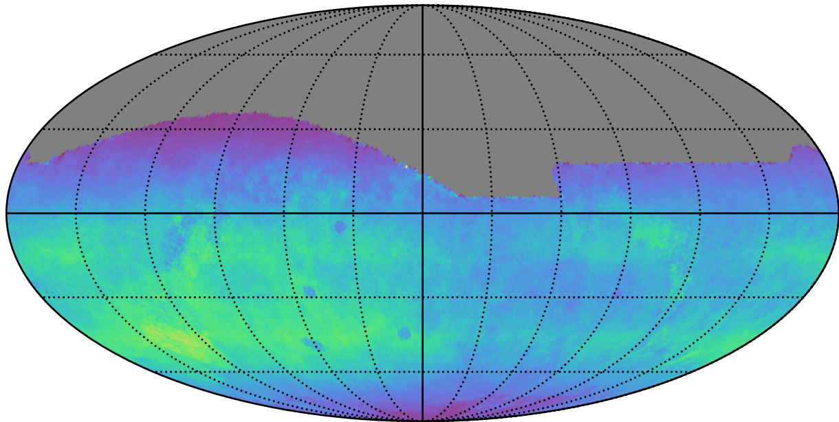
weather_cloudso0v3.5_10yrs All sky r band: Normalized Teff
