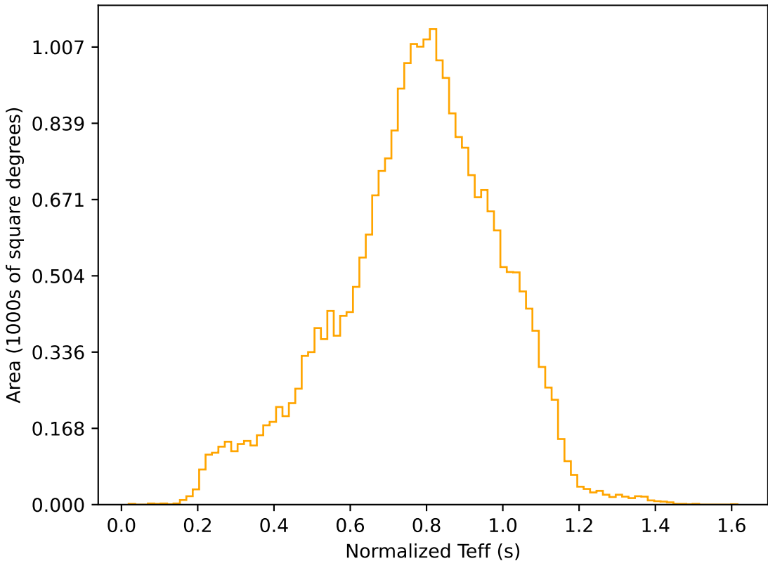
weather_cloudso0v3.5_10yrs All sky r band: Normalized Teff
