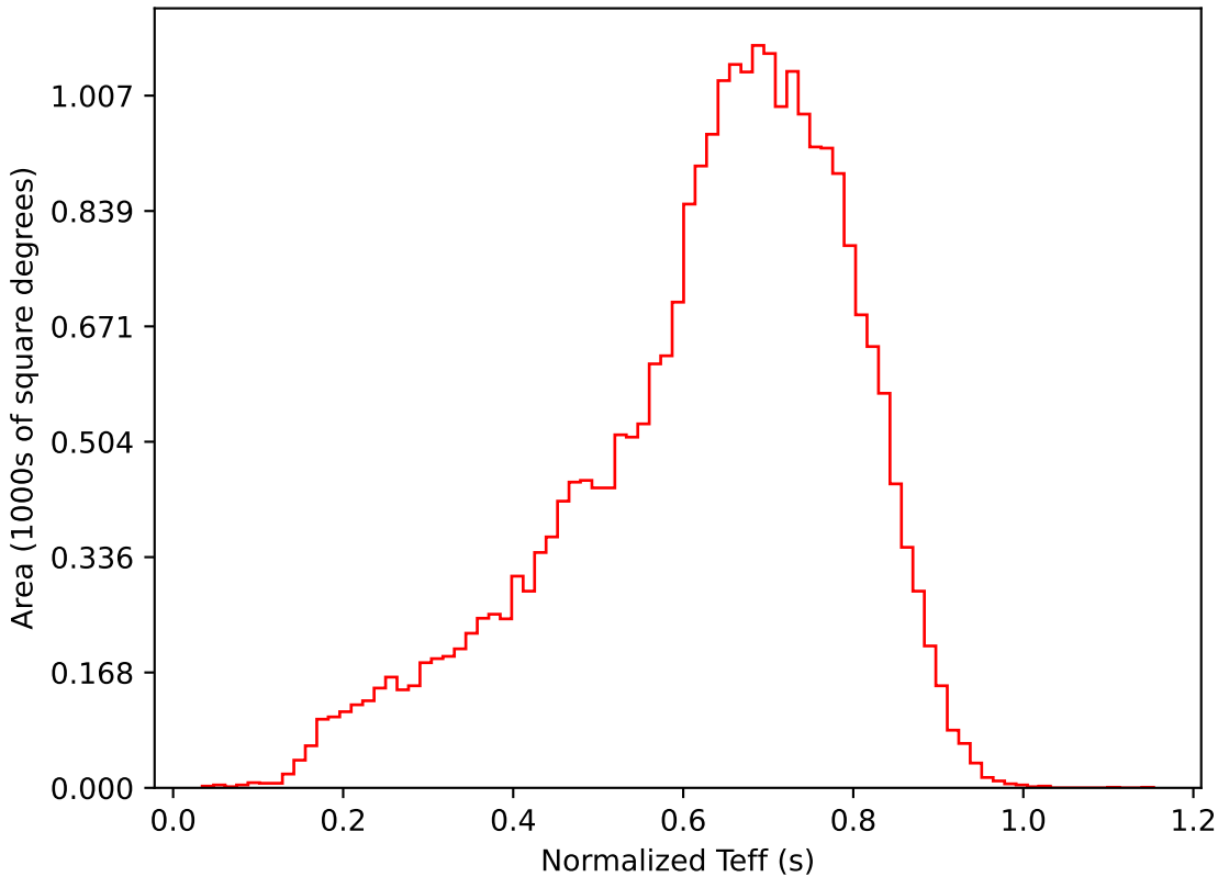
weather_cloudso0v3.5_10yrs All sky i band: Normalized Teff
