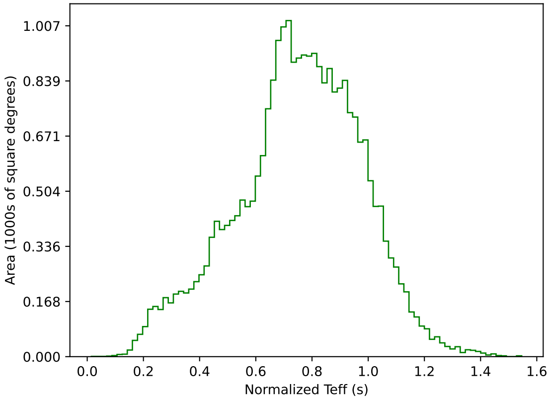
weather_cloudso0v3.5_10yrs All sky g band: Normalized Teff
