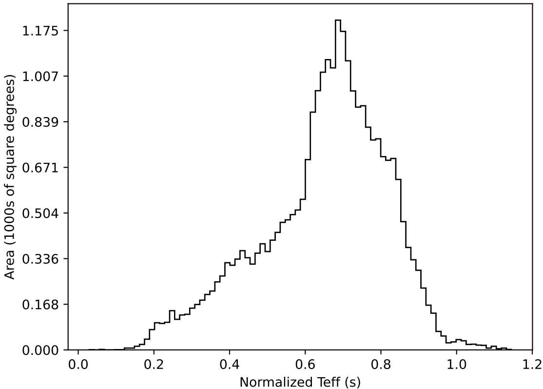
weather_cloudso0v3.5_10yrs All sky all bands: Normalized Teff
