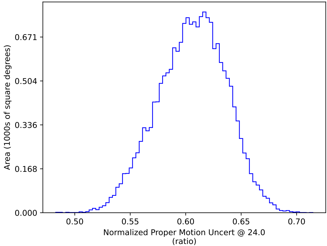
weather_cloudso0v3.5_10yrs WFD: Normalized Proper Motion Uncert @ 24.0
