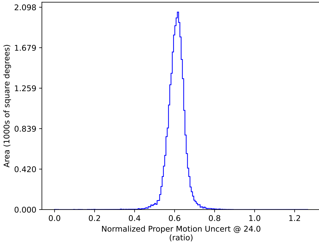
weather_cloudso0v3.5_10yrs All sky: Normalized Proper Motion Uncert @ 24.0
