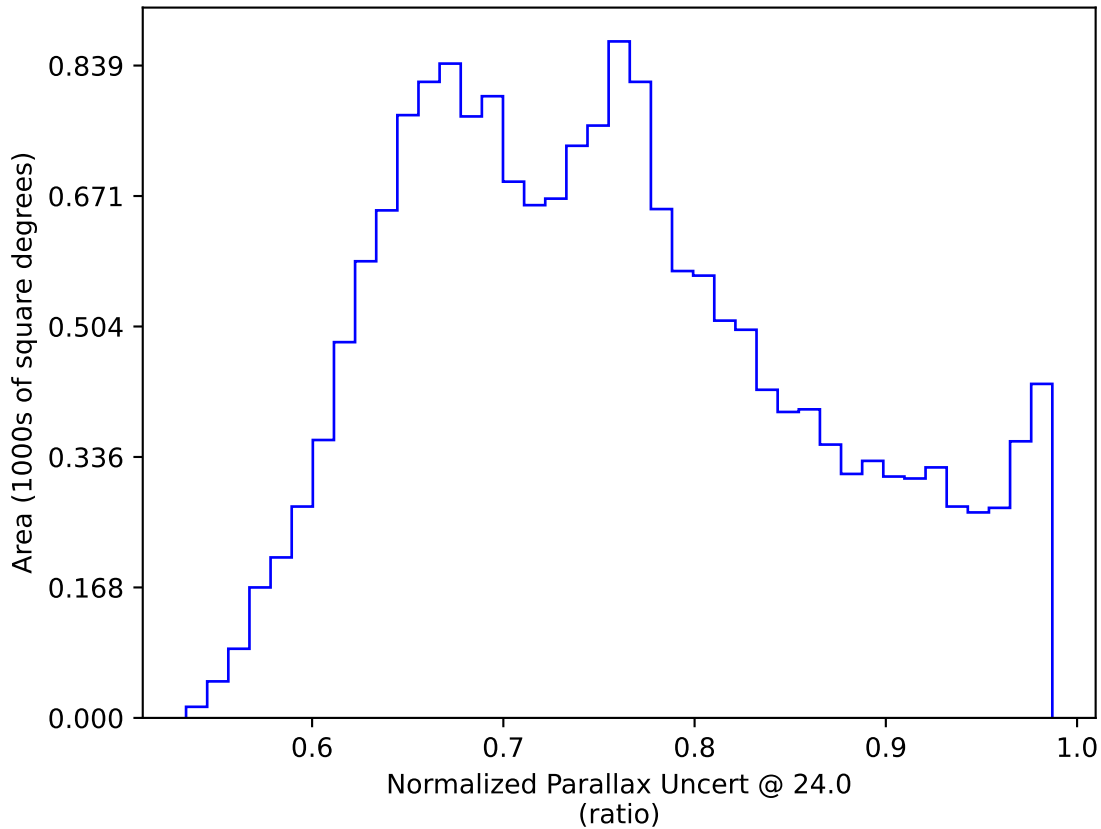
weather_cloudso0v3.5_10yrs WFD: Normalized Parallax Uncert @ 24.0
