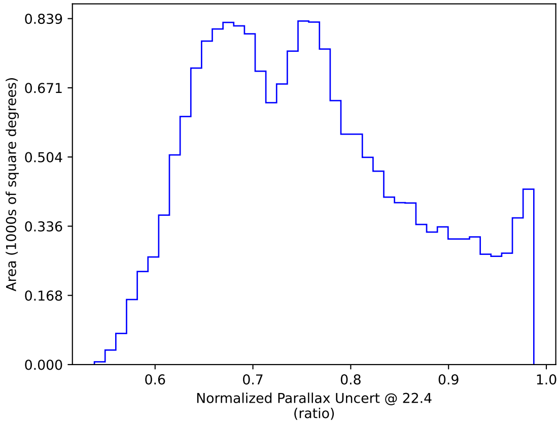
weather_cloudso0v3.5_10yrs WFD: Normalized Parallax Uncert @ 22.4
