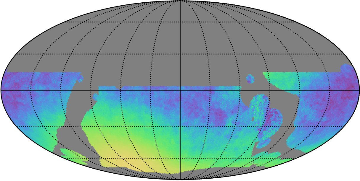
weather_cloudso0v3.5_10yrs WFD y band only: Normalized Parallax Uncert @ 21.3
