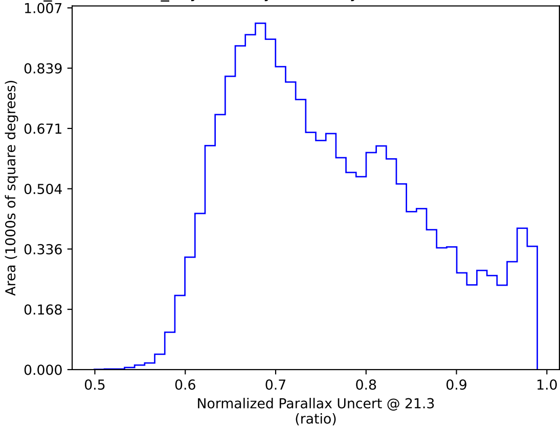
weather_cloudso0v3.5_10yrs WFD y band only: Normalized Parallax Uncert @ 21.3
