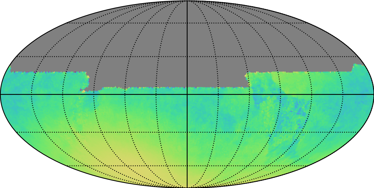
weather_cloudso0v3.5_10yrs All sky y band only: Normalized Parallax Uncert @ 21.3
