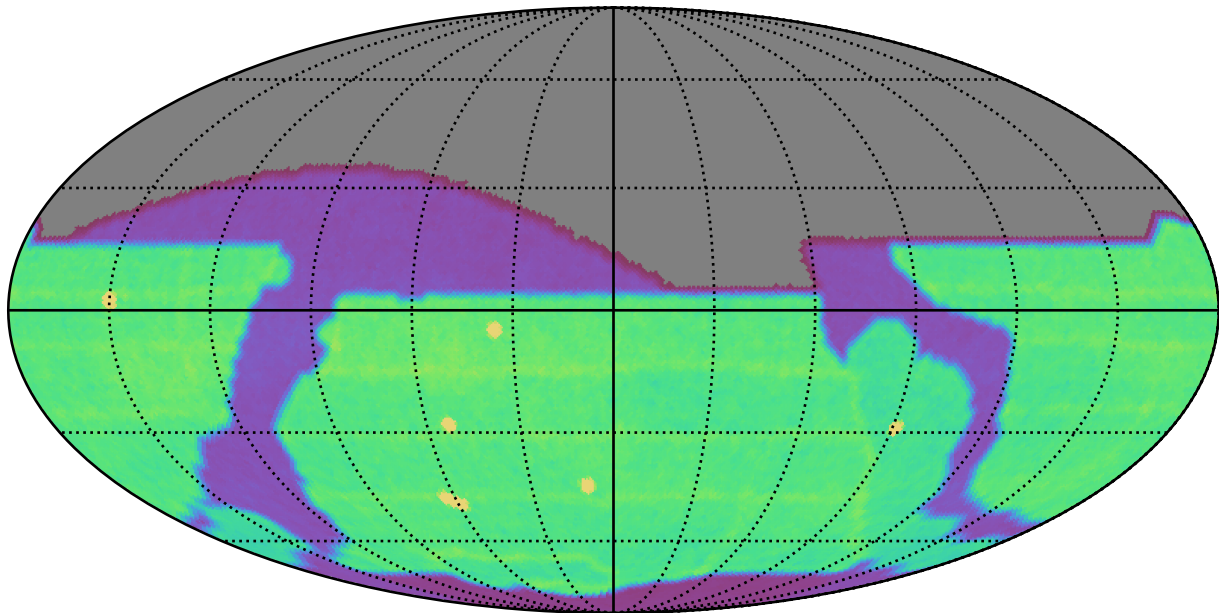
weather_cloudso0v3.5_10yrs All sky all bands: N Unique Nights
