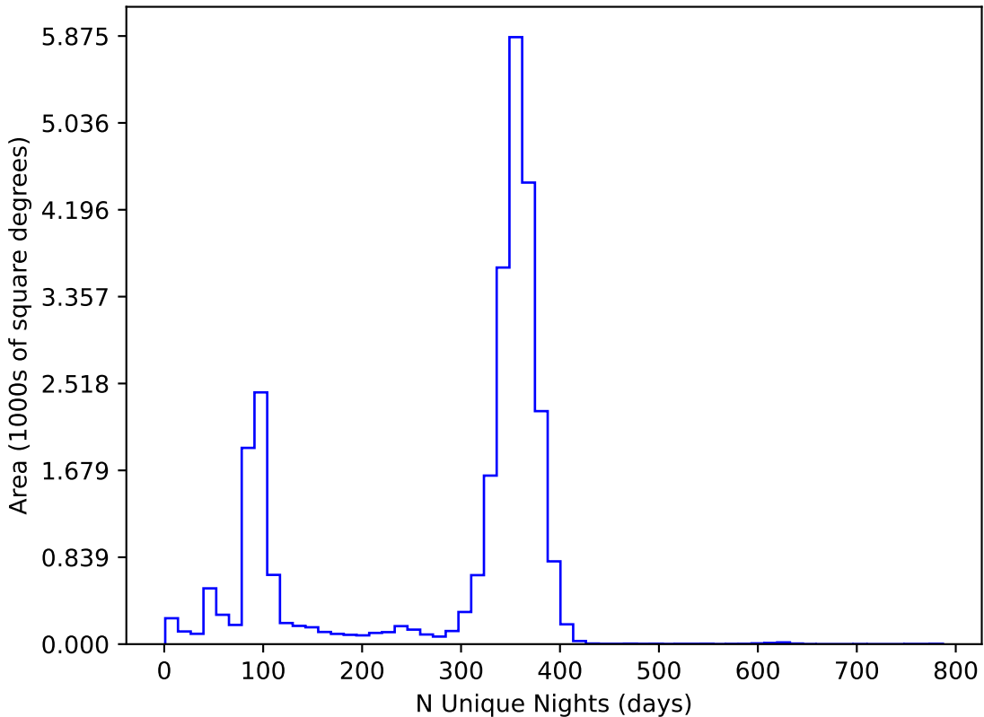
weather_cloudso0v3.5_10yrs All sky all bands: N Unique Nights
