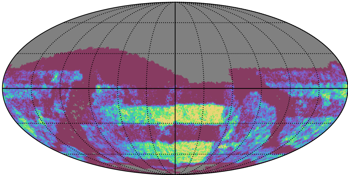
weather_cloudso0v3.5_10yrs Yr 3-4 z band: NVisits
