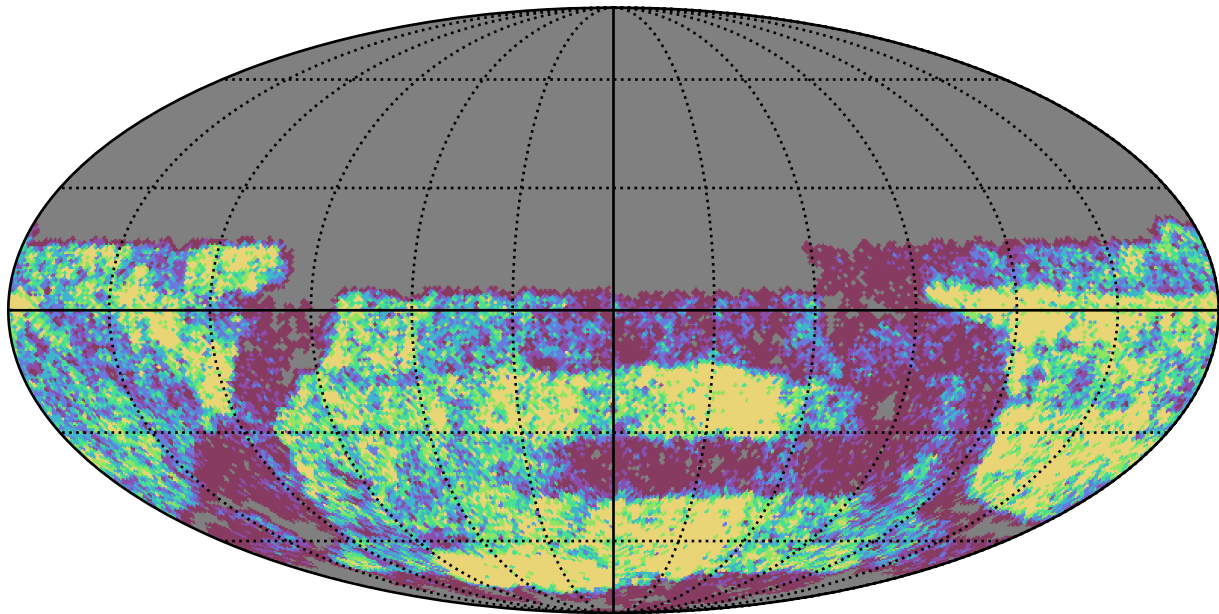
weather_cloudso0v3.5_10yrs Yr 3-4 u band: NVisits
