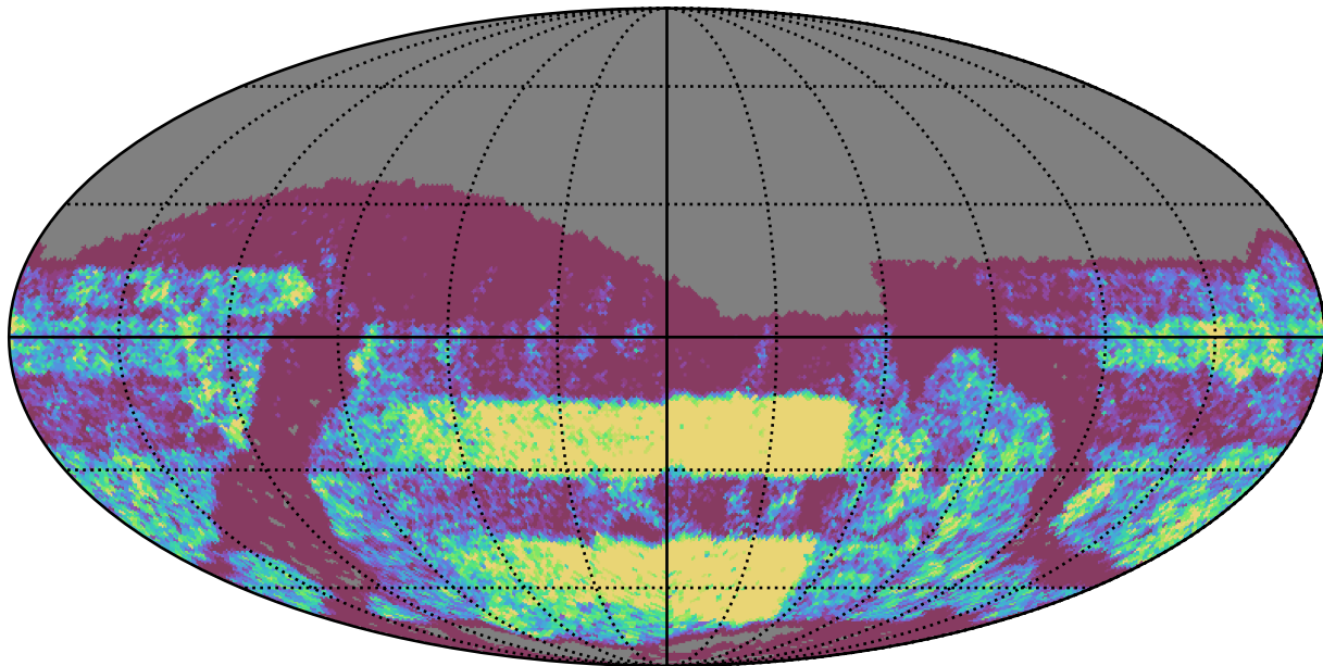
weather_cloudso0v3.5_10yrs Yr 3-4 i band: NVisits
