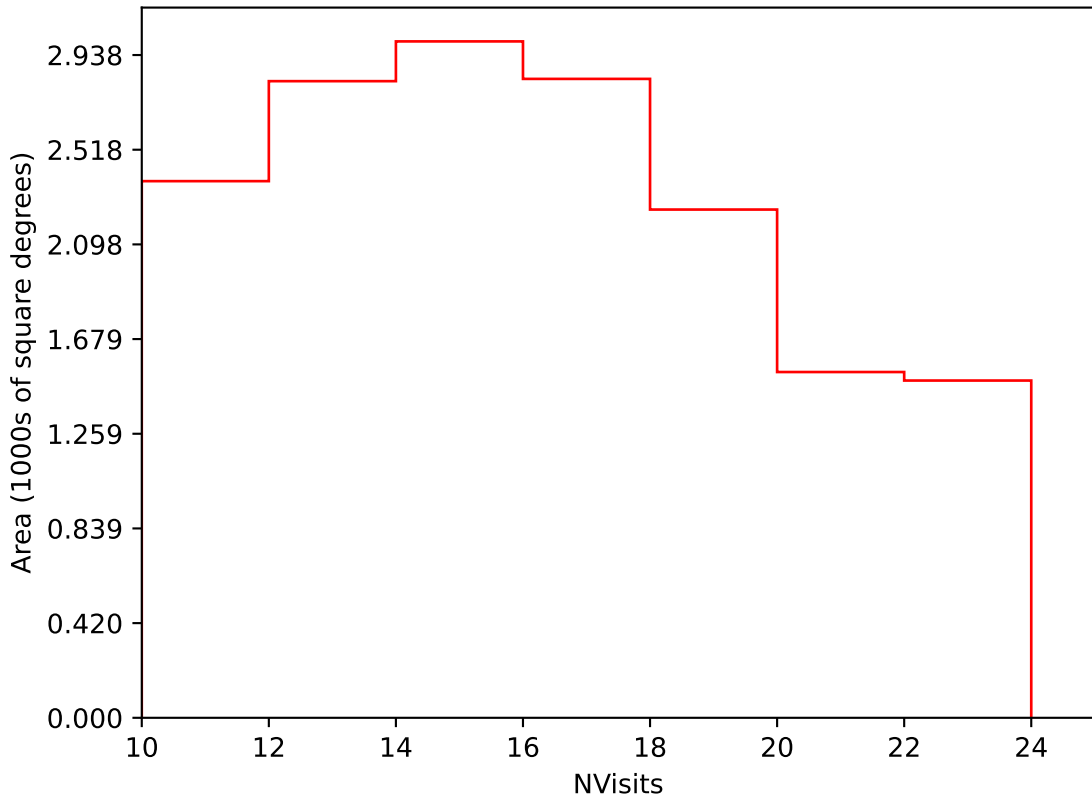
weather_cloudso0v3.5_10yrs Yr 3-4 i band: NVisits
