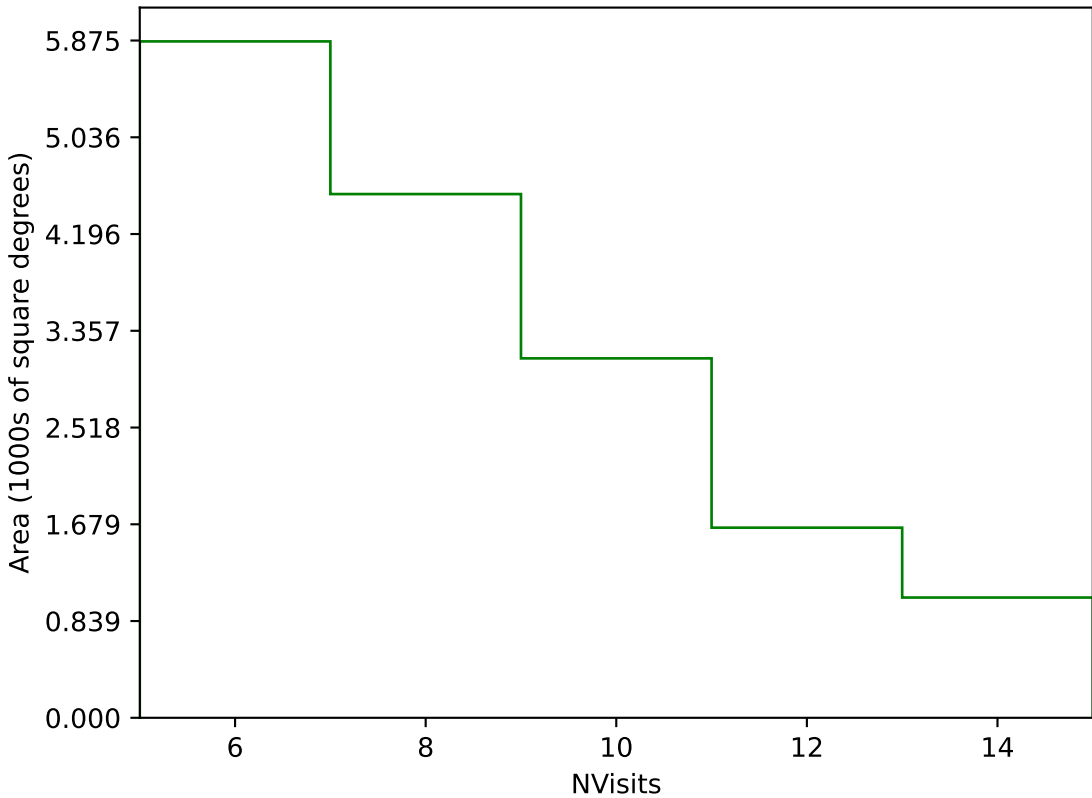
weather_cloudso0v3.5_10yrs Yr 3-4 g band: NVisits
