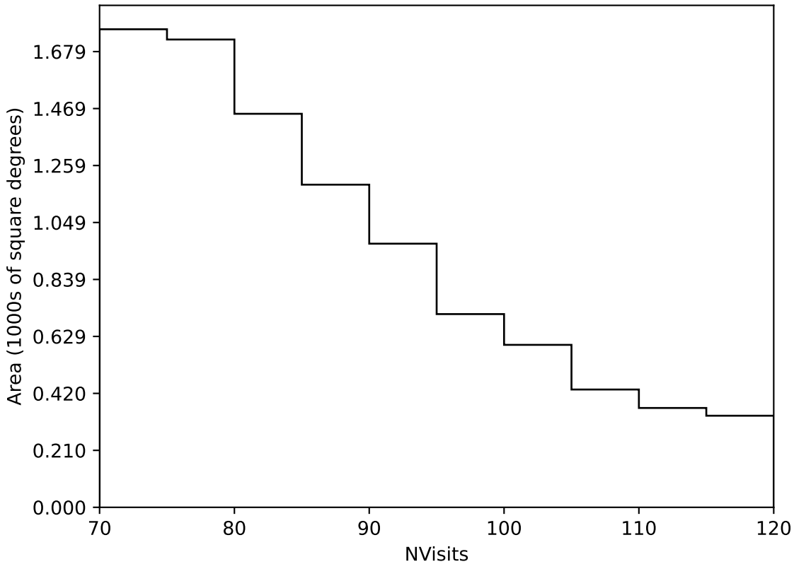
weather_cloudso0v3.5_10yrs Yr 3-4 all bands: NVisits
