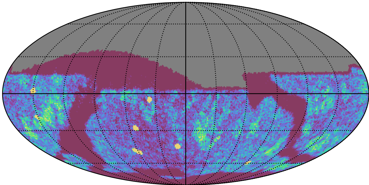
weather_cloudso0v3.5_10yrs Yr 1 z band: NVisits
