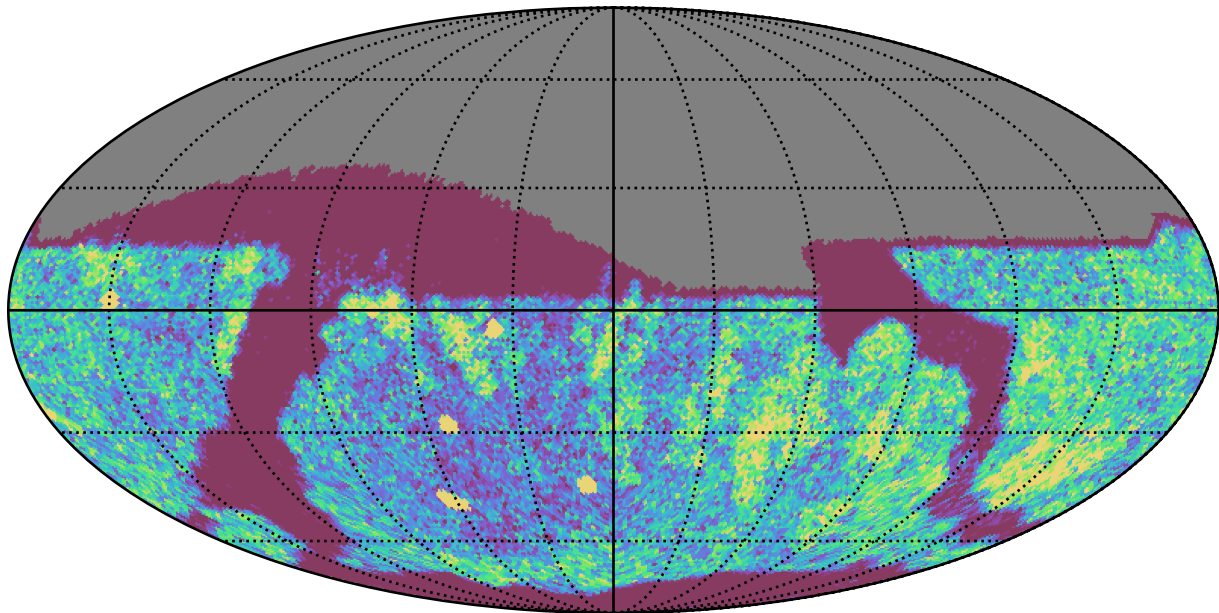
weather_cloudso0v3.5_10yrs Yr 1 r band: NVisits
