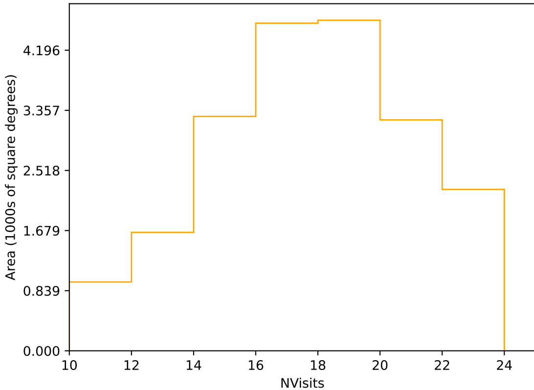
weather_cloudso0v3.5_10yrs Yr 1 r band: NVisits
