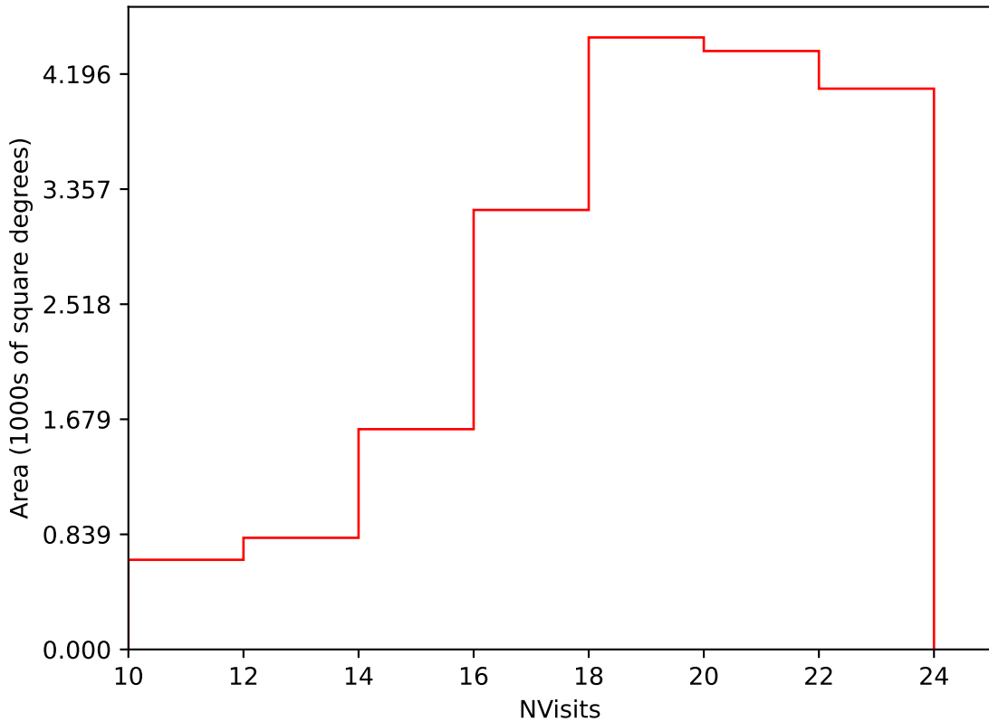
weather_cloudso0v3.5_10yrs Yr 1 i band: NVisits
