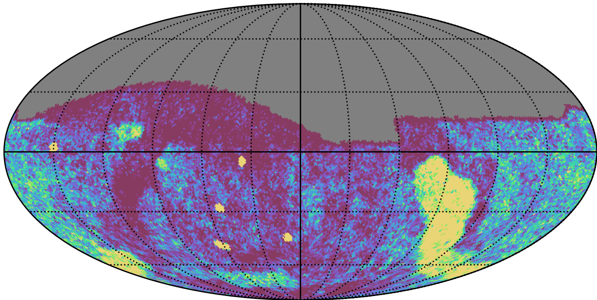
weather_cloudso0v3.5_10yrs Yr 1 g band: NVisits
