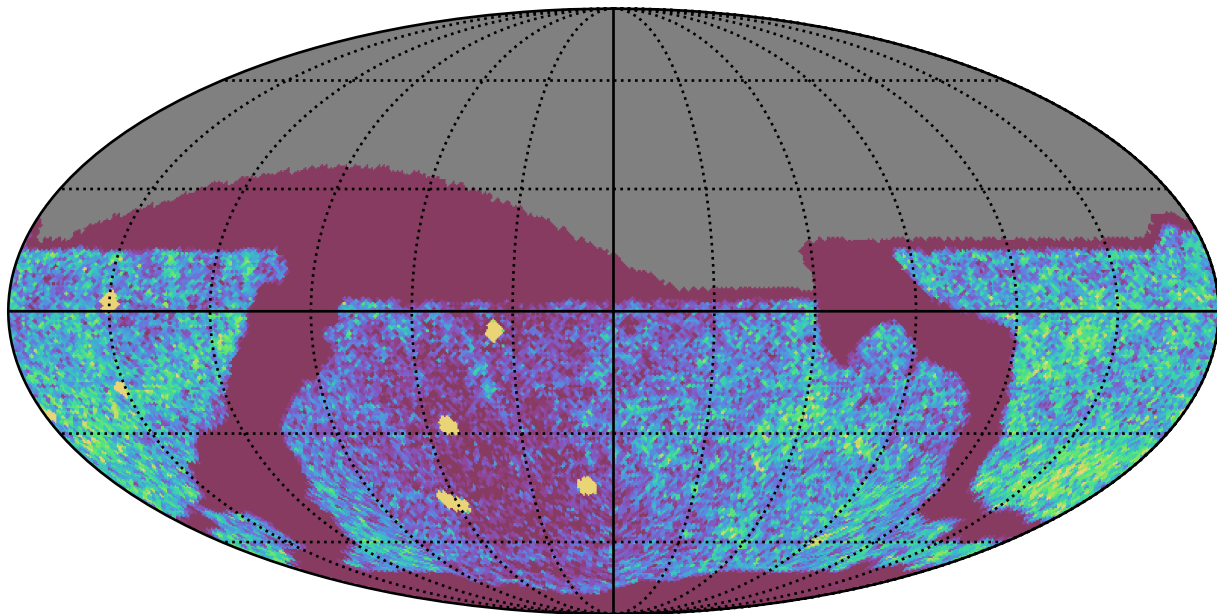
weather_cloudso0v3.5_10yrs Yr 1 all bands: NVisits
