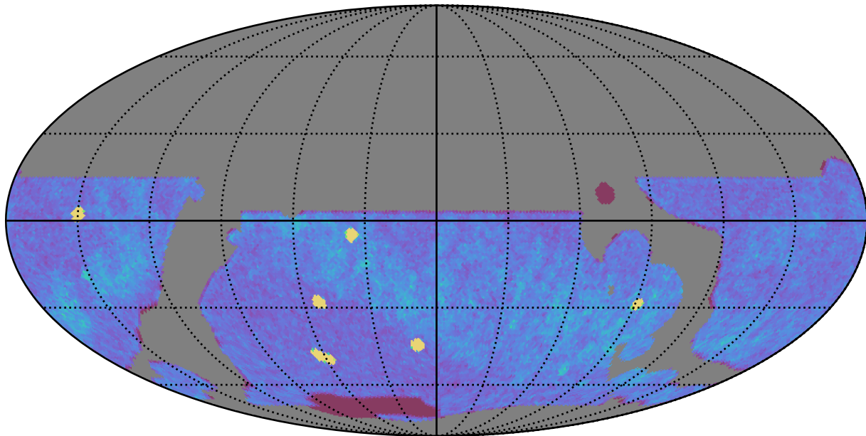
weather_cloudso0v3.5_10yrs WFD z band: NVisits
