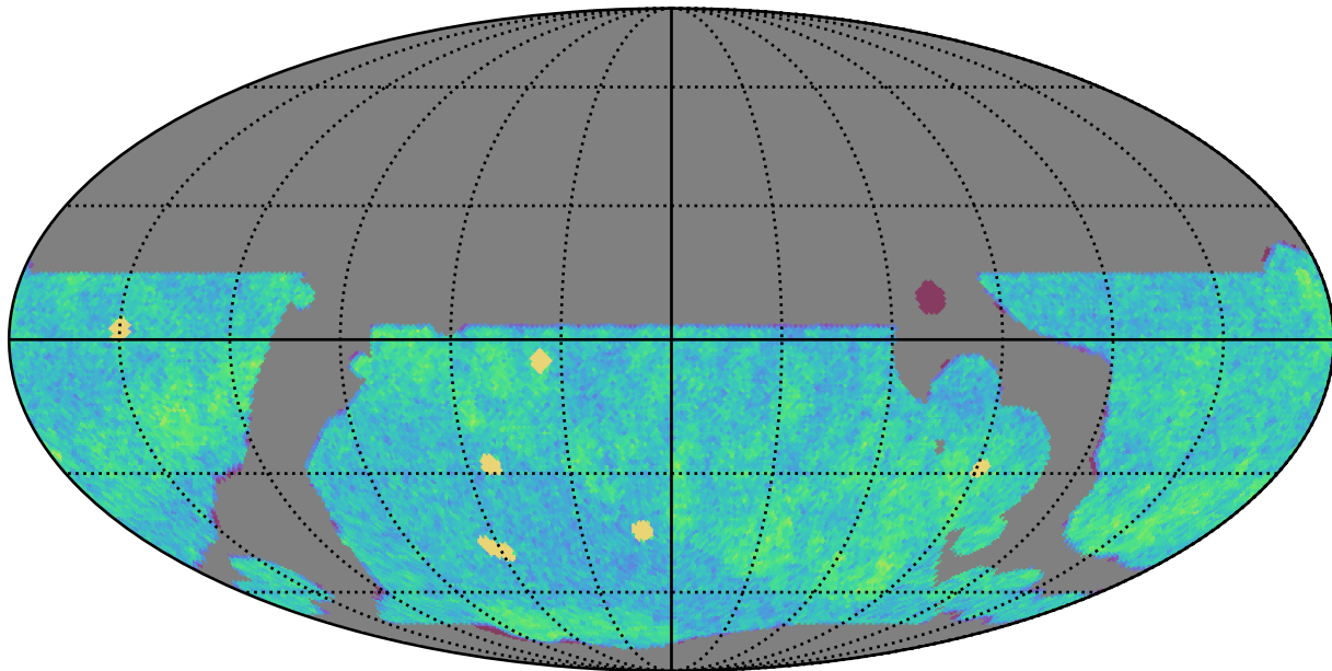
weather_cloudso0v3.5_10yrs WFD r band: NVisits
