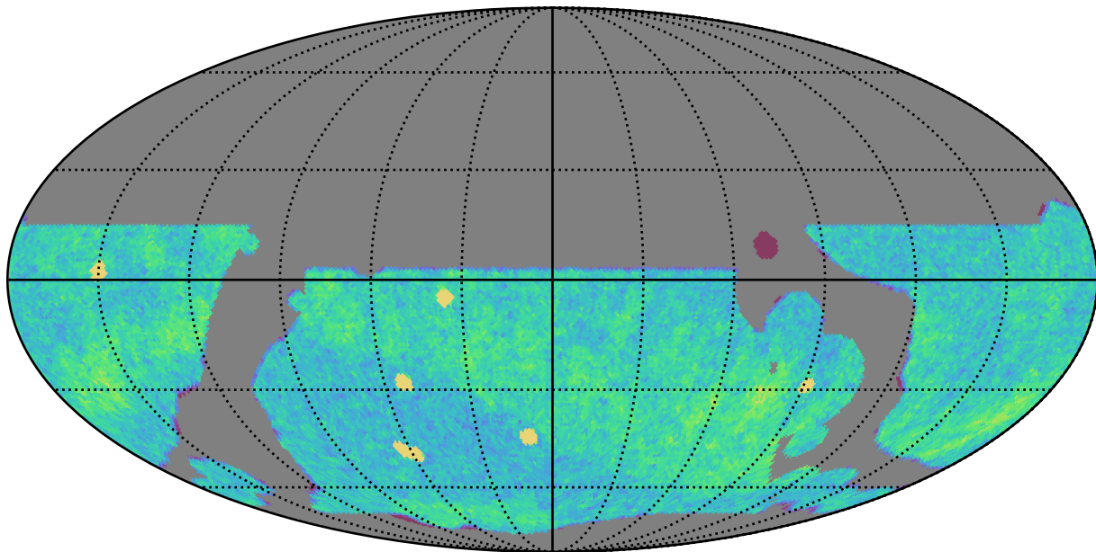
weather_cloudso0v3.5_10yrs WFD i band: NVisits
