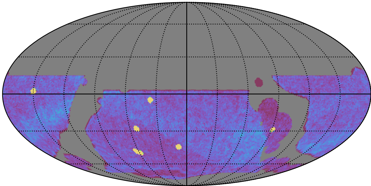
weather_cloudso0v3.5_10yrs WFD all bands: NVisits
