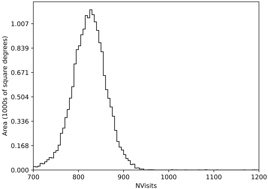
weather_cloudso0v3.5_10yrs WFD all bands: NVisits
