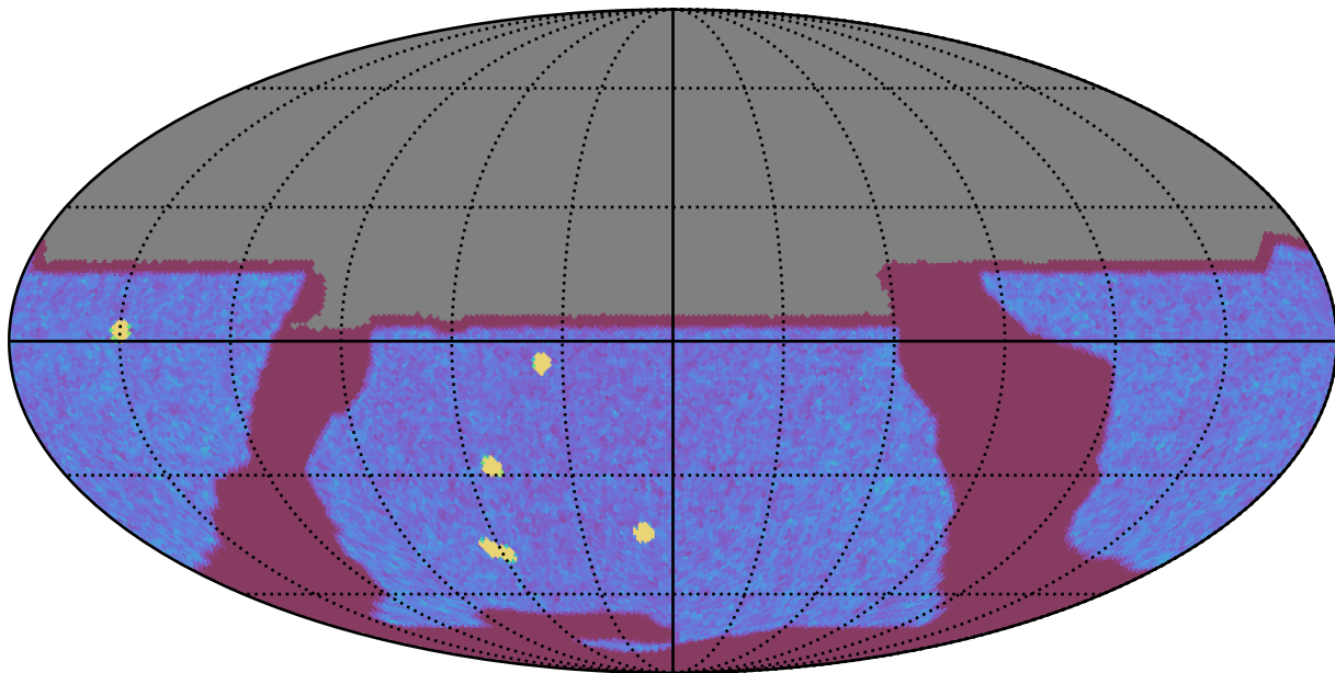
weather_cloudso0v3.5_10yrs All sky y band: NVisits
