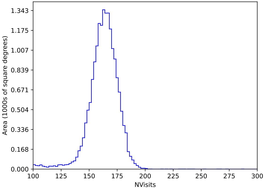
weather_cloudso0v3.5_10yrs All sky y band: NVisits
