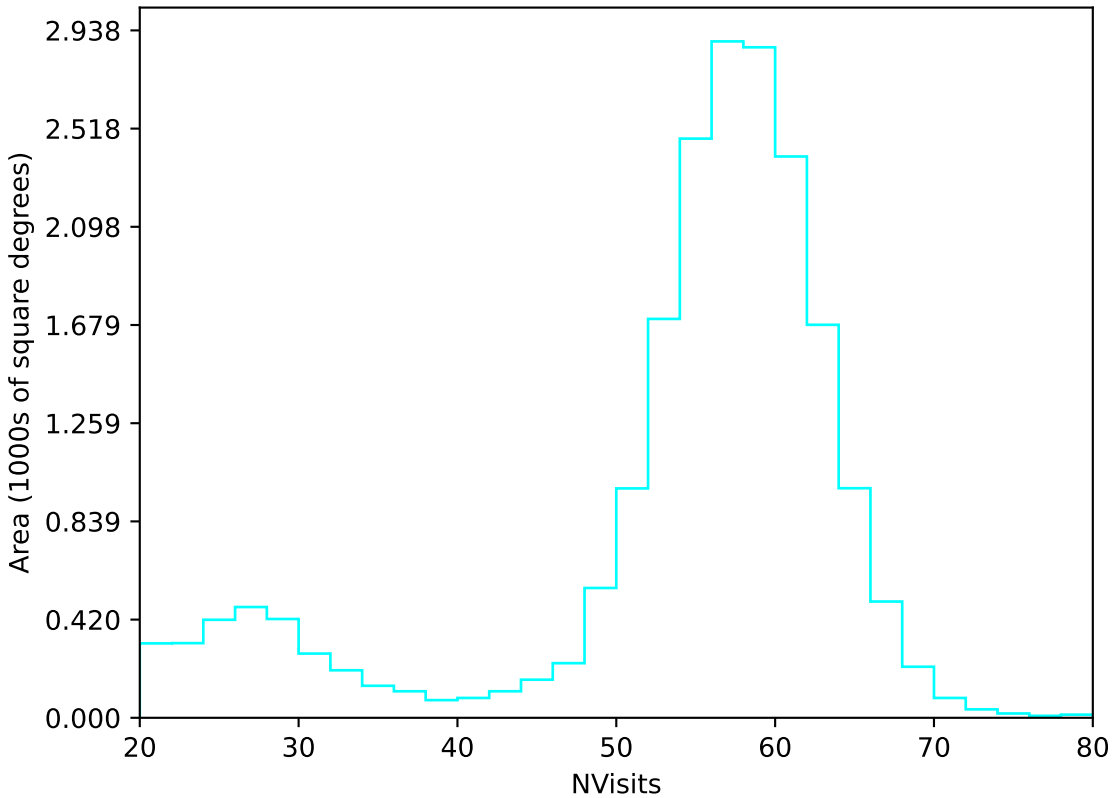
weather_cloudso0v3.5_10yrs All sky u band: NVisits
