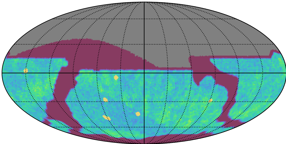
weather_cloudso0v3.5_10yrs All sky r band: NVisits
