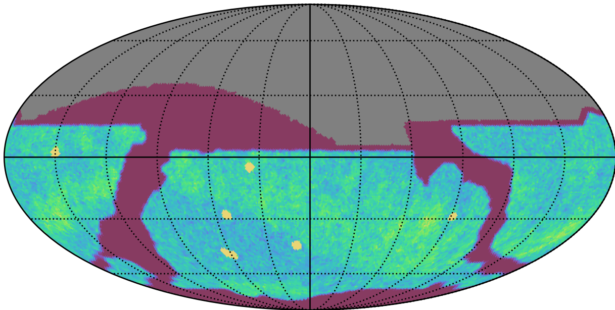
weather_cloudso0v3.5_10yrs All sky i band: NVisits
