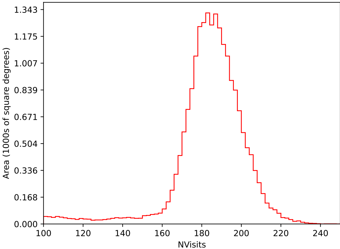
weather_cloudso0v3.5_10yrs All sky i band: NVisits
