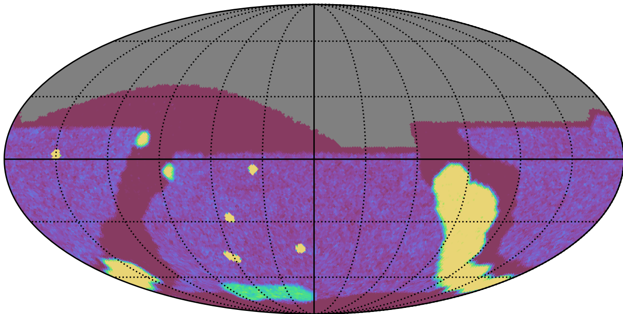
weather_cloudso0v3.5_10yrs All sky g band: NVisits
