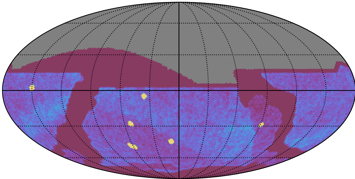
weather_cloudso0v3.5_10yrs All sky all bands: NVisits
