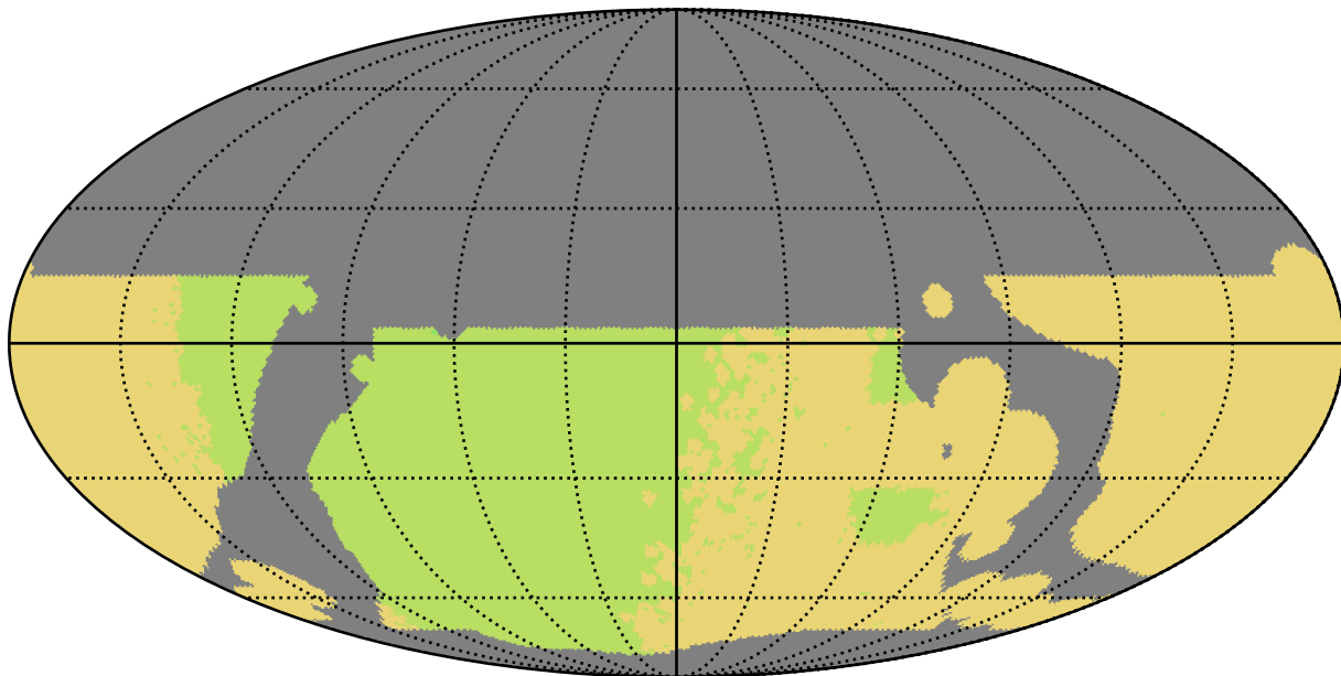
weather_cloudso0v3.5_10yrs WFD all bands: NSeasons
