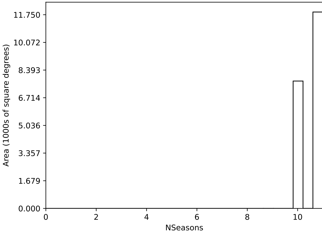
weather_cloudso0v3.5_10yrs WFD all bands: NSeasons
