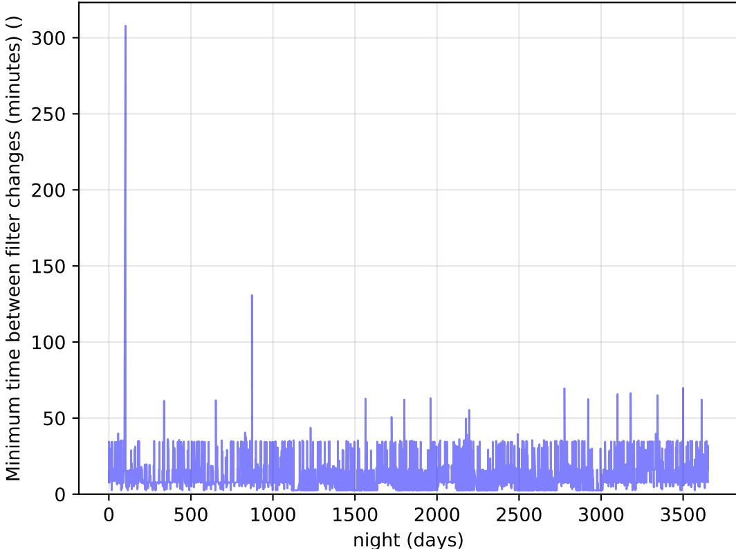
weather_cloudso0v3.5_10yrs Per Night: Minimum time between filter changes (minutes)
