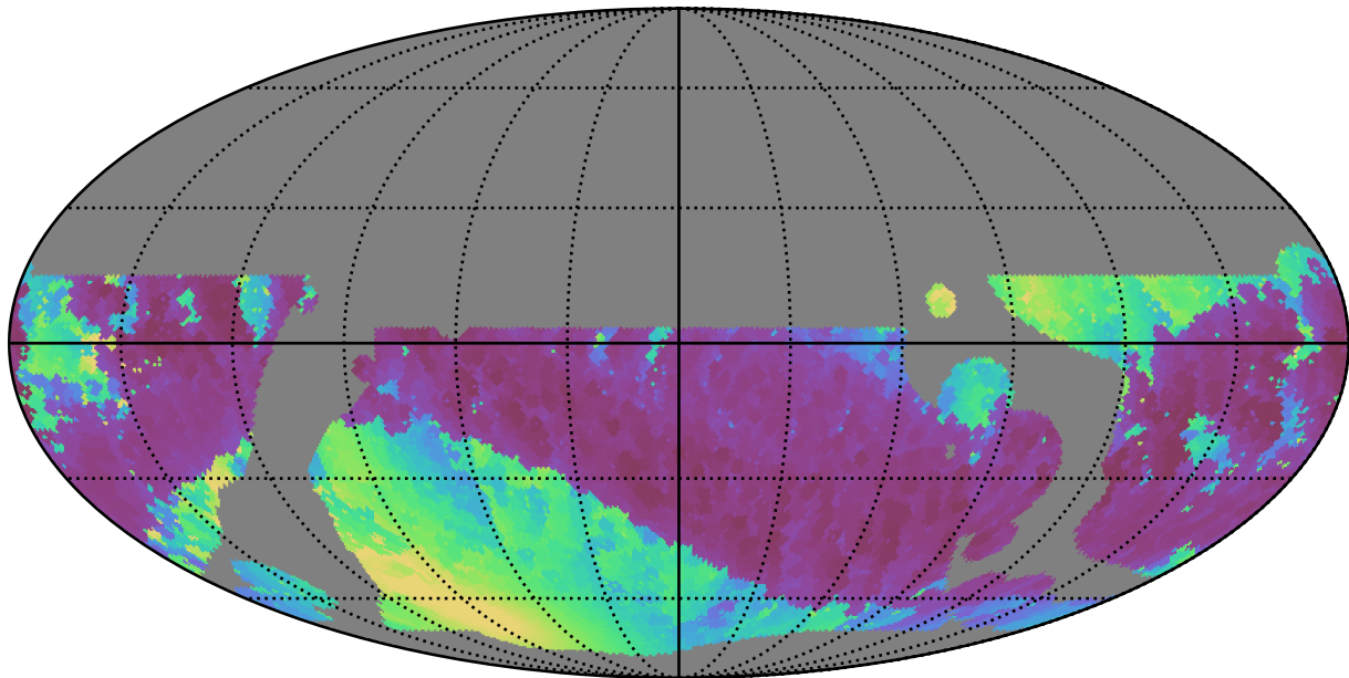
weather_cloudso0v3.5_10yrs WFD z band: Min solarElong
