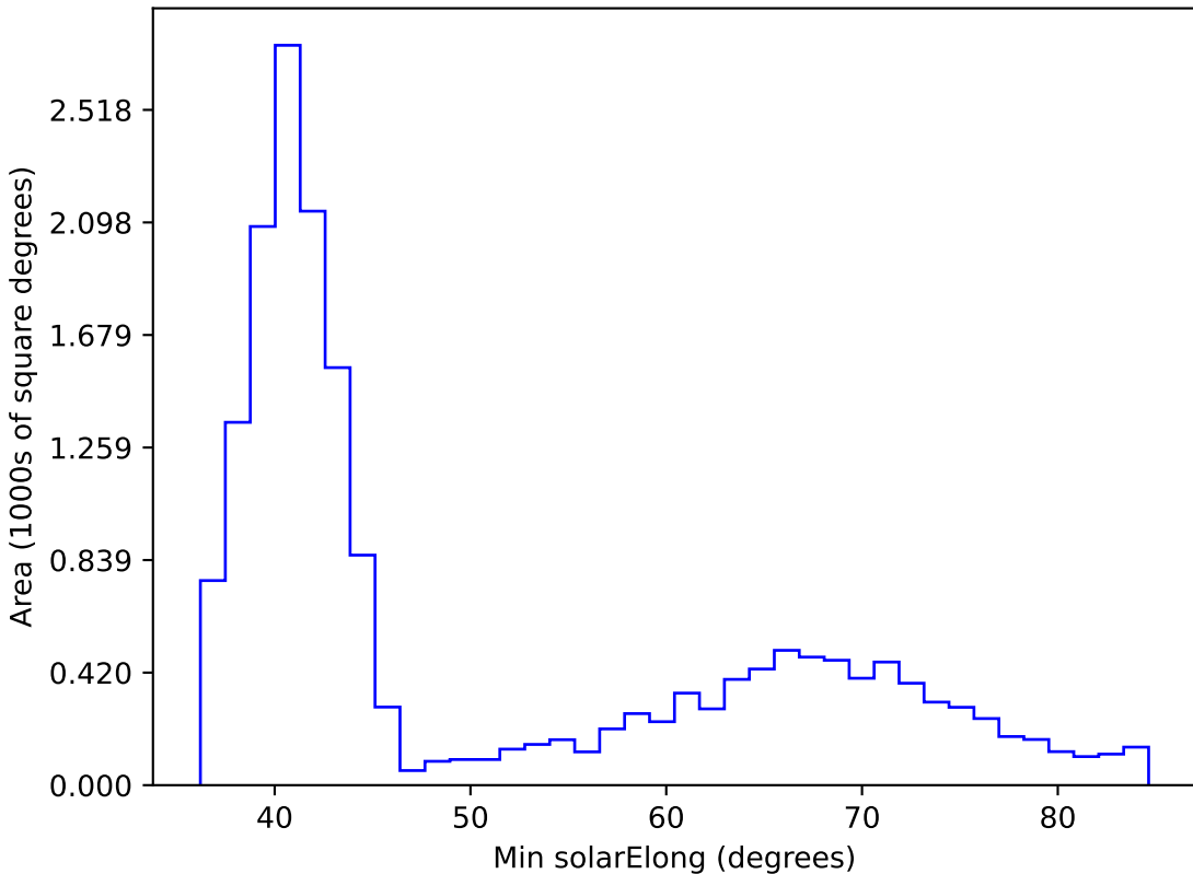
weather_cloudso0v3.5_10yrs WFD z band: Min solarElong
