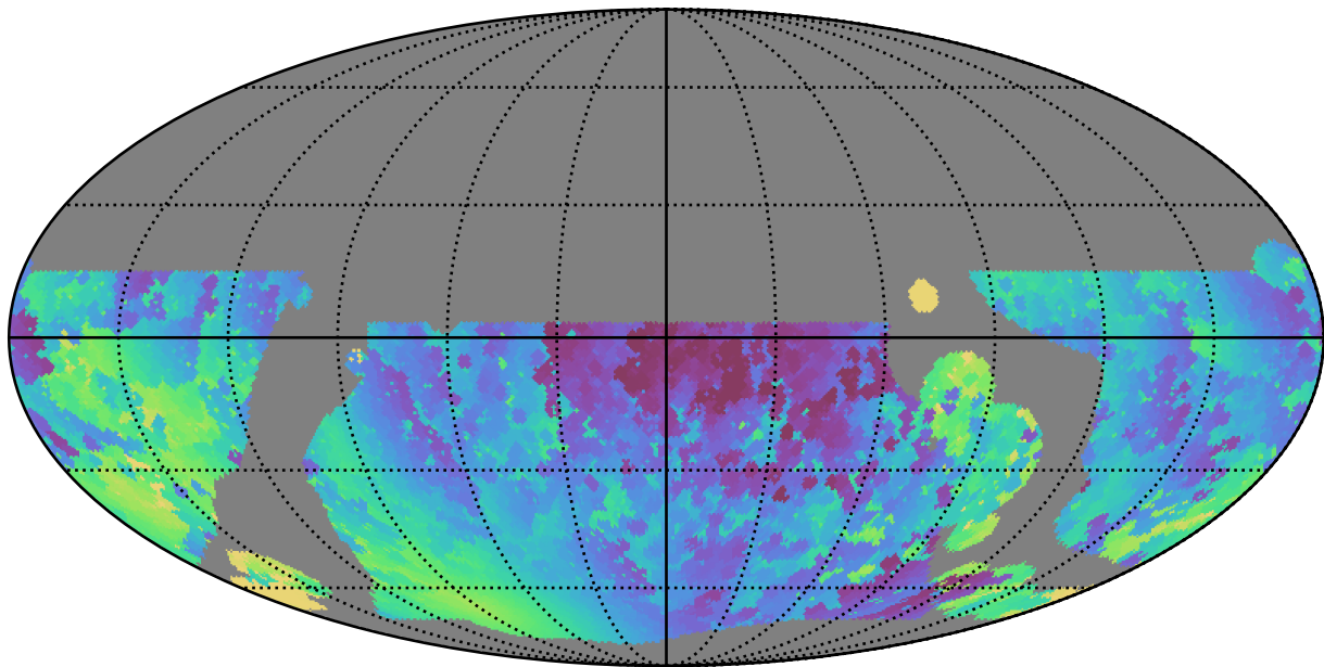
weather_cloudso0v3.5_10yrs WFD y band: Min solarElong
