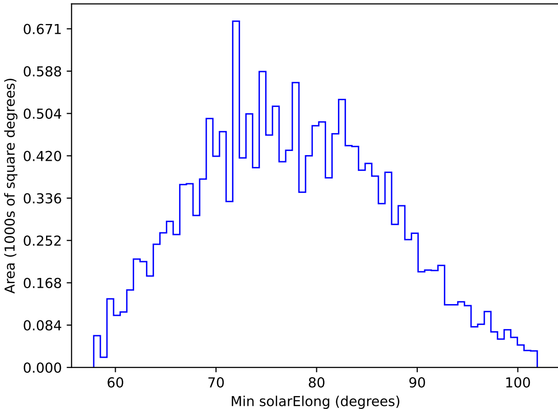
weather_cloudso0v3.5_10yrs WFD u band: Min solarElong
