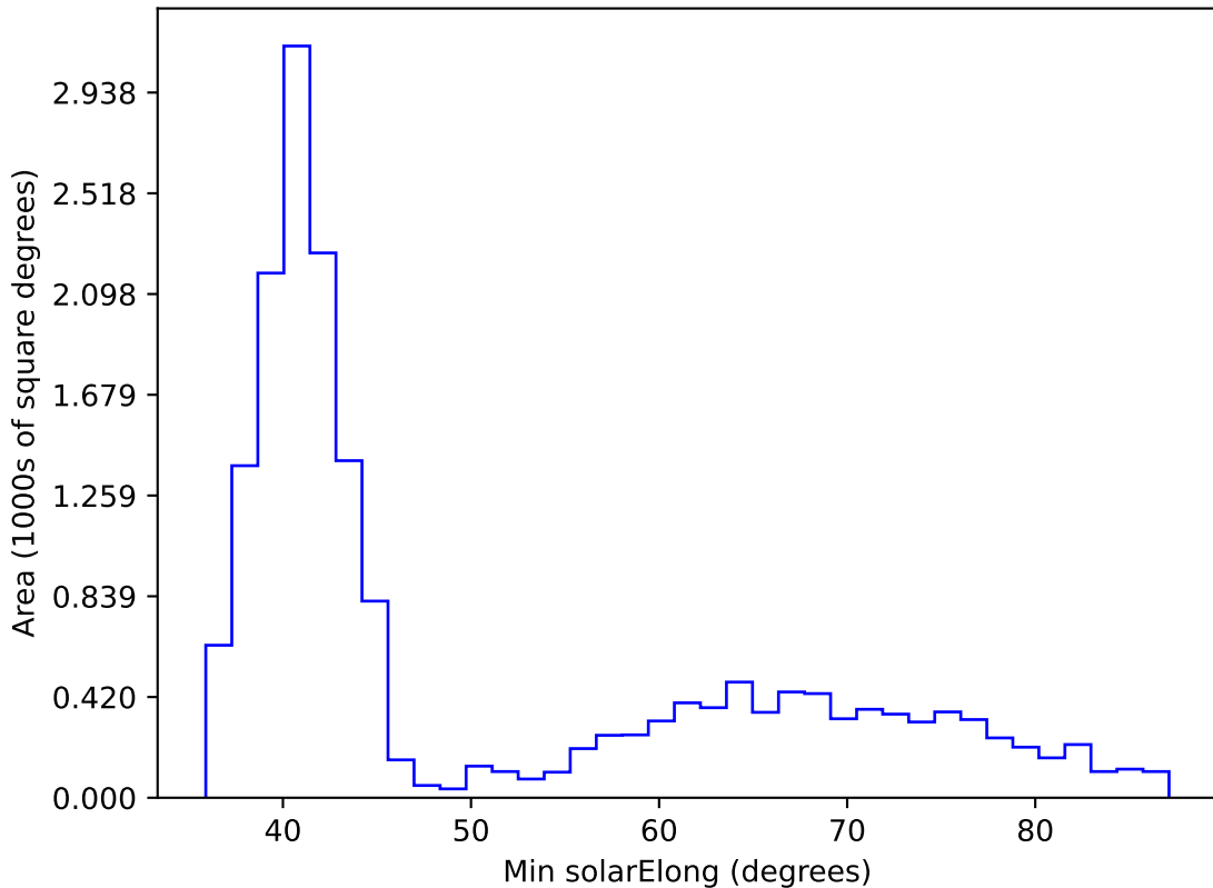
weather_cloudso0v3.5_10yrs WFD r band: Min solarElong
